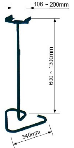
DSP-014 • 座地喇叭支架 • Speaker Floor Stand • For Surround Speaker
